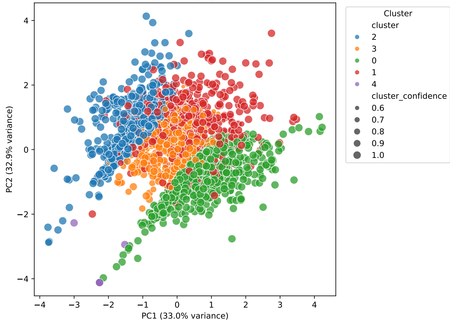
GMM Cluster Separability by PCA Projection
